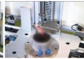
置入波形墊圈 Place in wave washer
